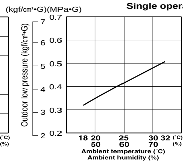
Single operation (Unit C or D)
