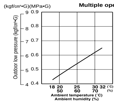
Multiple operation (Unit A+B)
