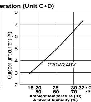
Multiple operation (Unit C+D)
