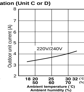
Single operation (Unit C or D)
