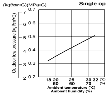
Single operation (Unit A or B)
