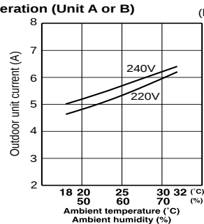
Single operation (Unit A or B)
