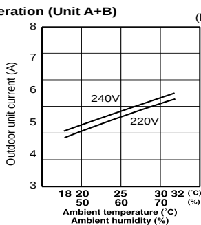
Multiple operation (Unit A+B)
