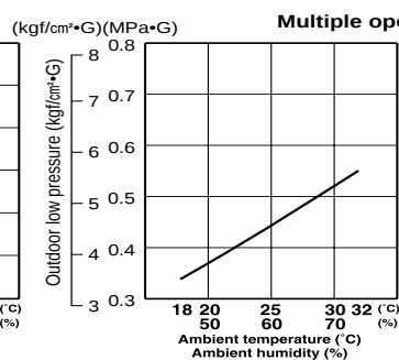
Multiple operation (Unit C+D)
